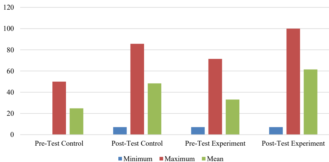
Figure 1. Descriptive Statistics Data Visualization
